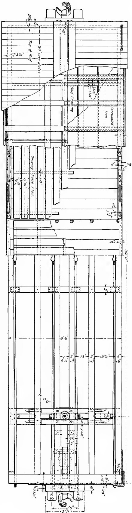
Fig. 264. Sectional Plan of Roof and Underframe. FRUIT-CAR BODY. CINCINNATI, NEW ORLEANS & TEXAS PACIFIC RAILWAY. Length, 35 ft. 3 ins. Capacity, 40,000 lbs. Weight, 34,800 lbs.
